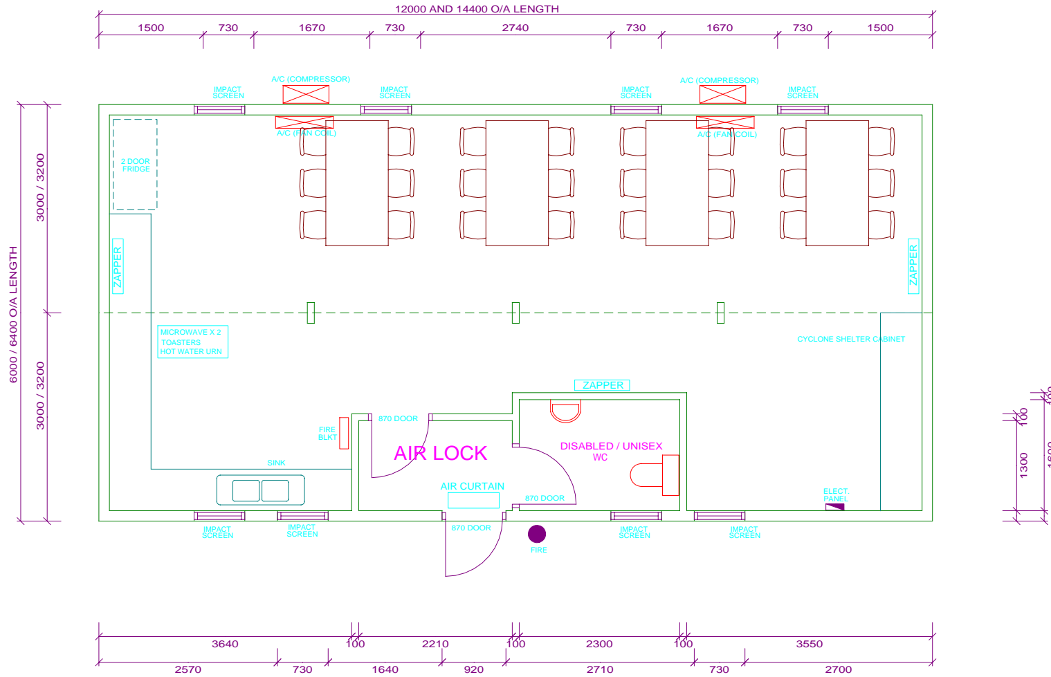
CYCLONE SHELTER SCALE 1:50 COMPLEXED ARRANGEMENT
