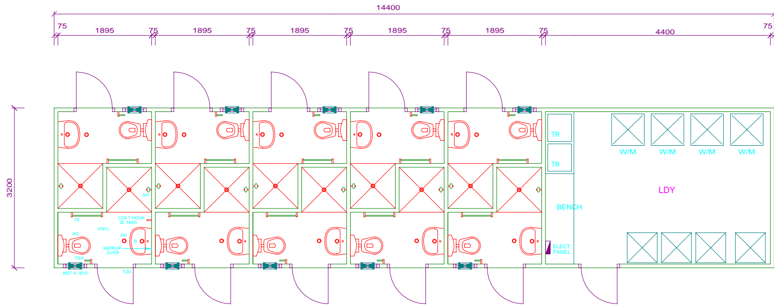
AMENITIES BLOCK SCALE 1:50 SHOWER - WC/LDY ARRANGEMNTS
